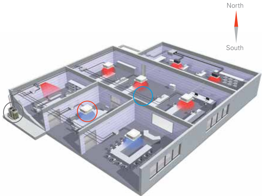
Refrigerant piping
